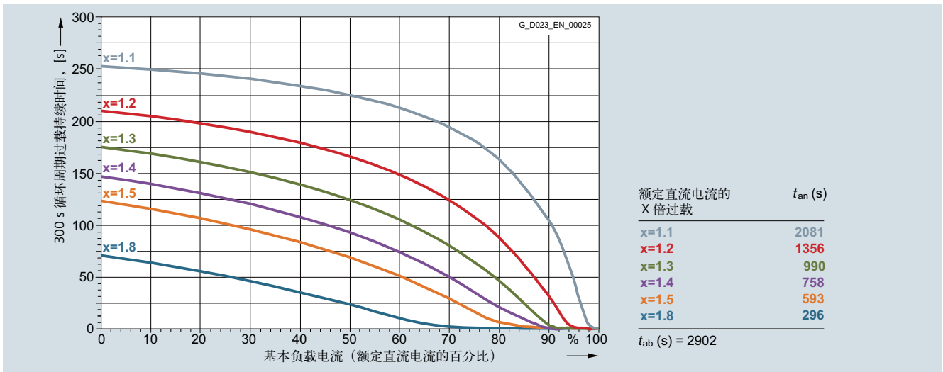
6RA8025-6DS22-0AA0 60 A/ 两象限运行, 400 V; 6RA8025-6FS22-0AA0 60 A/ 两象限运行, 480 V, 6RA8025-6GS22-0AA0 60 A/ 两象限运行, 575 V
